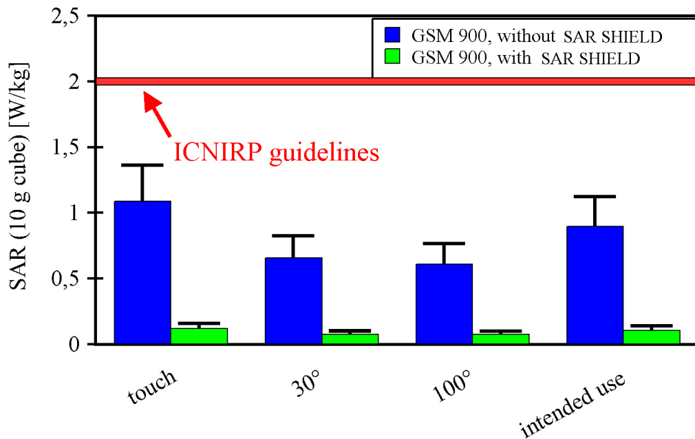
Fig. 8: The measured SAR values for GSM 900 using the Nokia 5110 in comparison to the ICNIRP Guidelines without and with the SAR SHIELD (left hand position).
