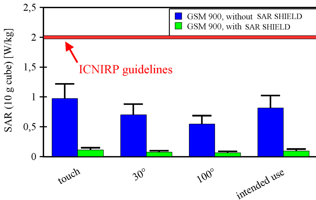
Fig. 9: The measured SAR values for GSM 900 using the Nokia 5110 in comparison to the ICNIRP Guidelines without and with the SAR SHIELD (right hand position).
